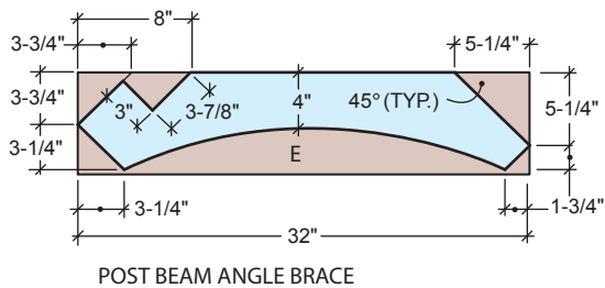
FIG. A SHADING STRUCTURE DETAILS
