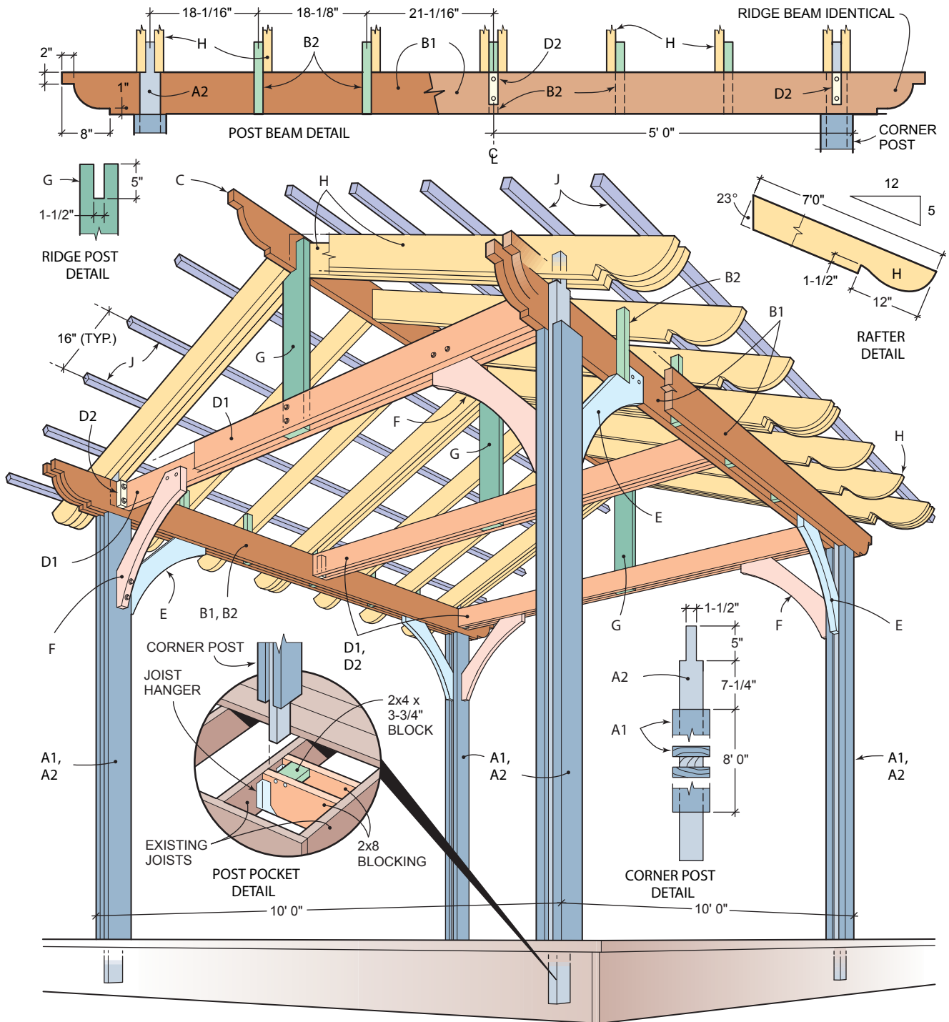
FIG. A SHADING STRUCTURE DETAILS
